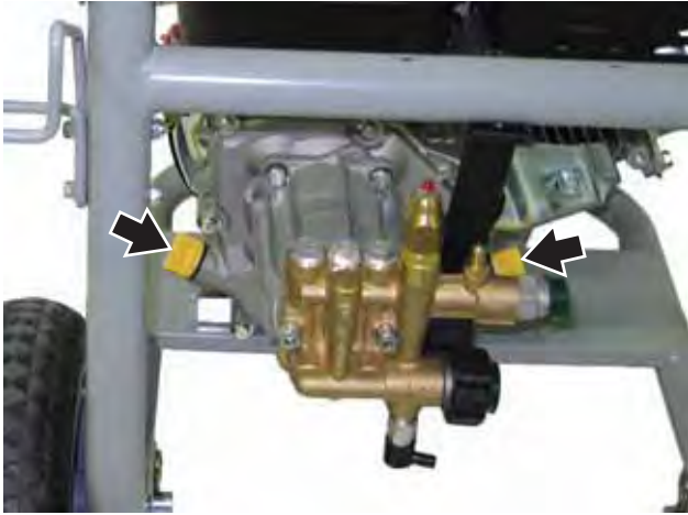
Figure 38 – Oil Fill Plug/Dipstick – WP3000
