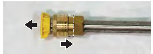
Figure 34 – Installing a Nozzle
