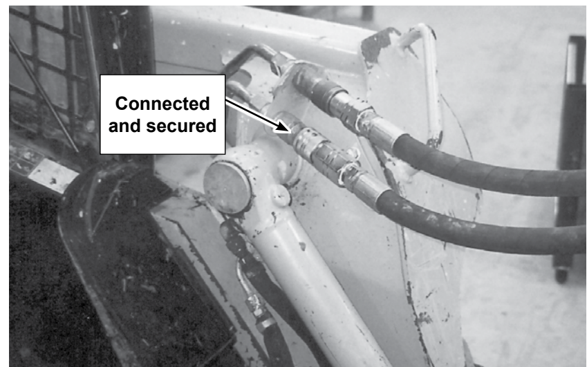
Fig. 6 HYDRAULICS
