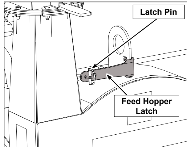
Fig. 12 FEED HOPPER LATCH SECURED
