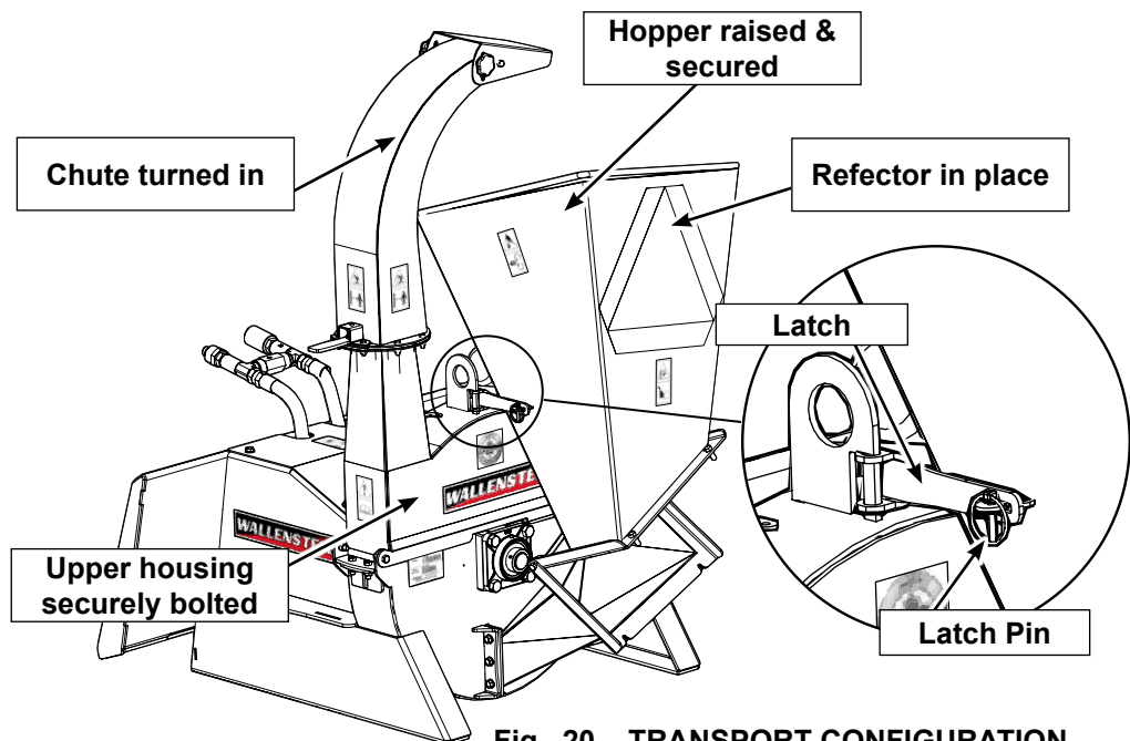
Fig. 20 TRANSPORT CONFIGURATION
