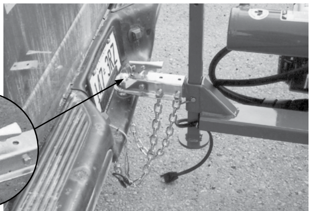
Fig. 4 RETAINER/STAND/SAFETY CHAIN
