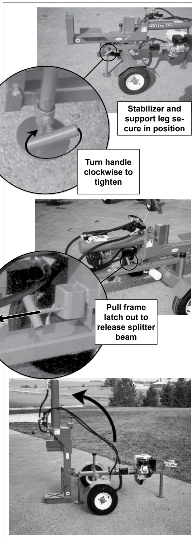
Fig. 14 VERTICAL SPLITTING
