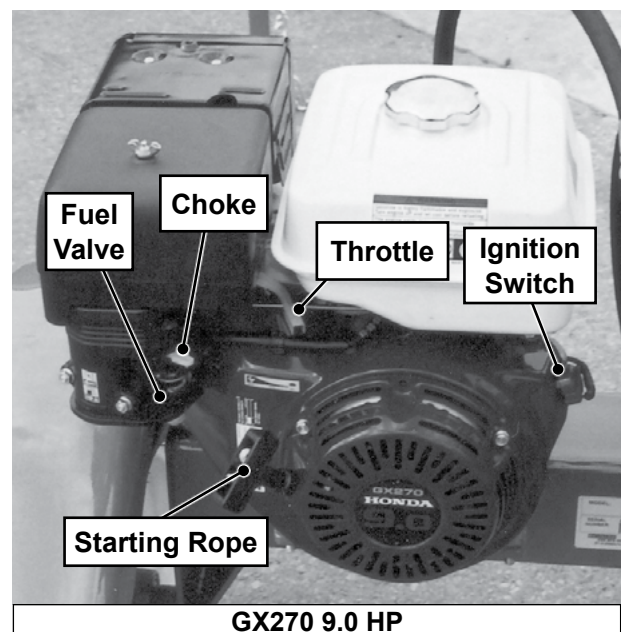
Fig. 7 ENGINE CONTROLS
