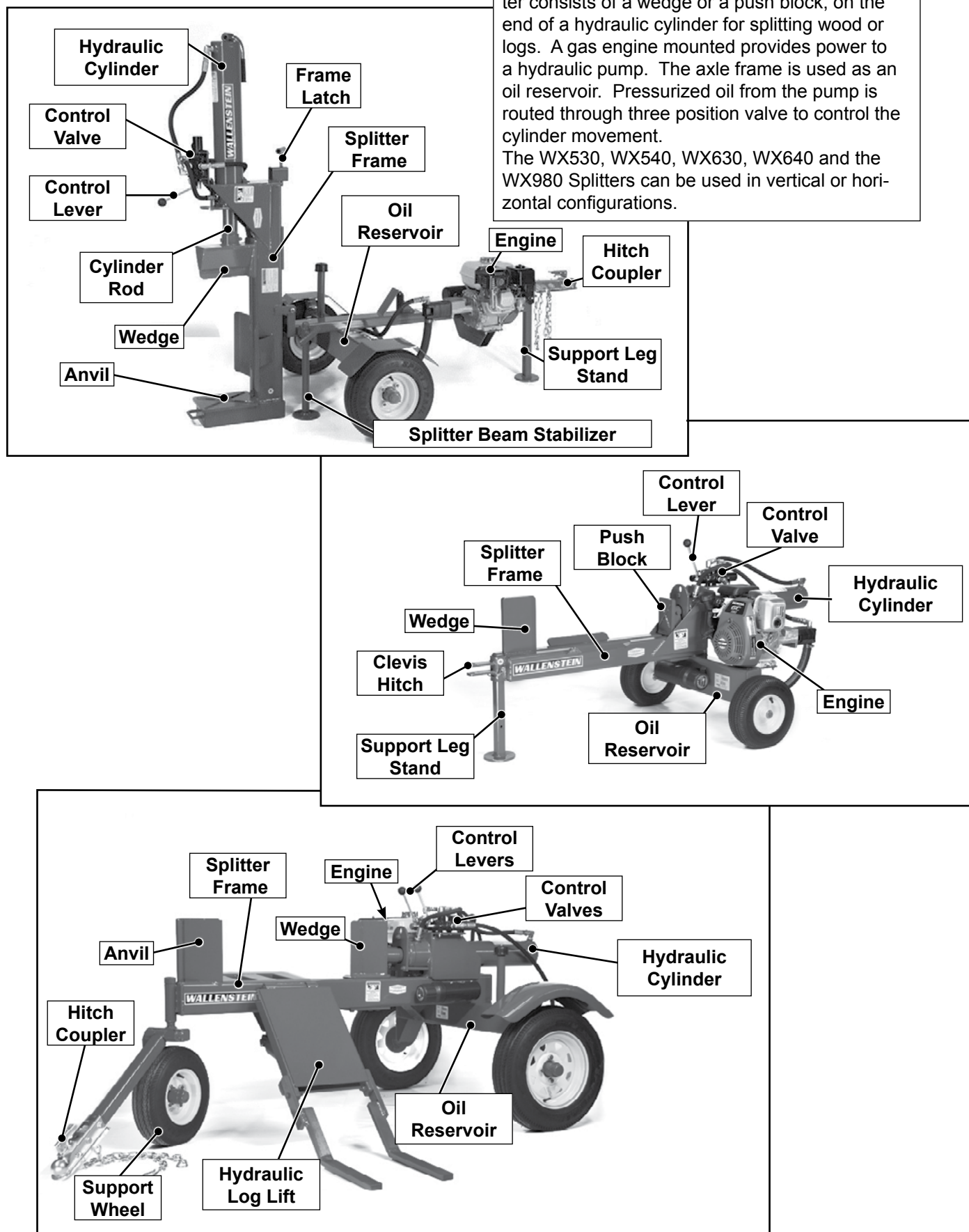
Fig. 1 MACHINE COMPONENTS
