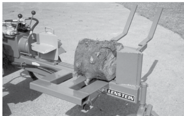
Cradle Raised and Log Positioned
