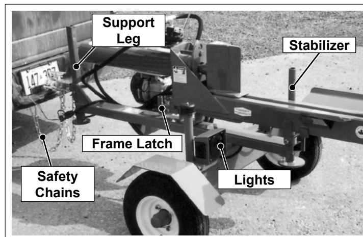
Fig. 16 TRANSPORTING
