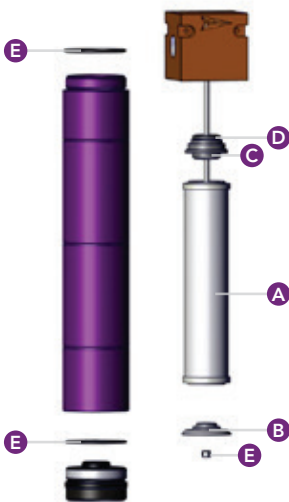
Figure 5 : Activated Carbon Filter
