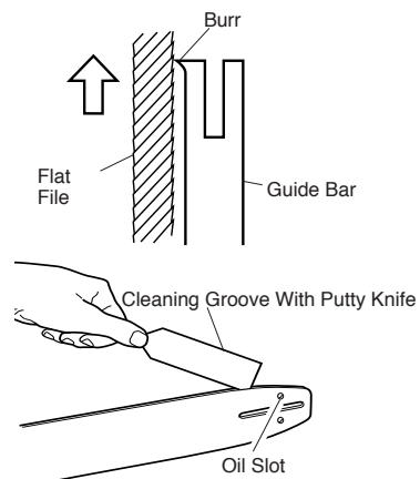
Figure 22 - Guide Bar Maintenance
