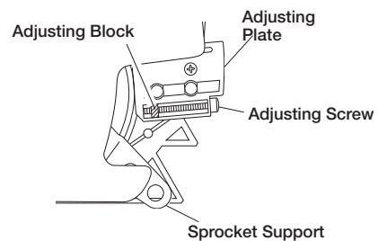
Figure 3 - Part Locations For Assembling Guide Bar
