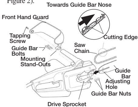
Figure 2 - Assembling Guide Bar, Chain, and Hand Guard
