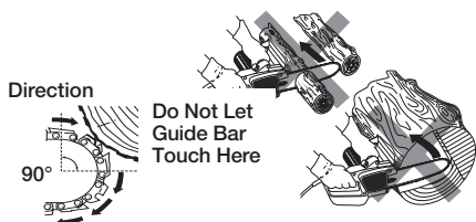
Figure 1 - Kickback Hazard Example: Do Not Let Nose of Guide Bar Touch Object While Chain is Moving
