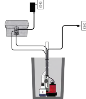
Recommended Installation
