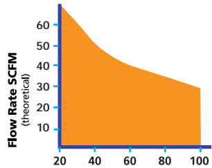
1/2" Maxline (.48 Inside Diameter) at 150 psi, 10 psi pressure drop
