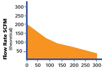
3/4" Maxline (.80 Inside Diameter) at 150 psi, 10 psi pressure drop
