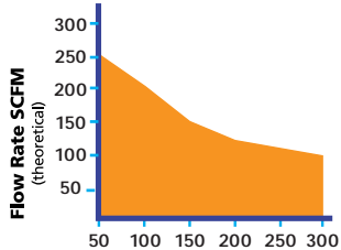
1" Maxline (1.02 Inside Diameter) at 150 psi, 10 psi pressure drop
