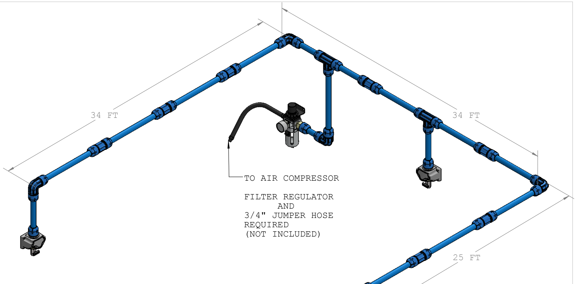
3/4 FASTPIPE KIT # F28075
