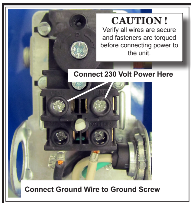
Fig. 1 Electrical Connections for Model 1312101159
