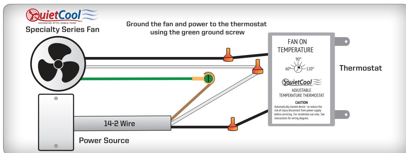
Figure 3.2A: Thermostat Wiring
