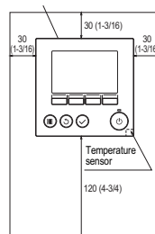
External dimensions of remote controller
