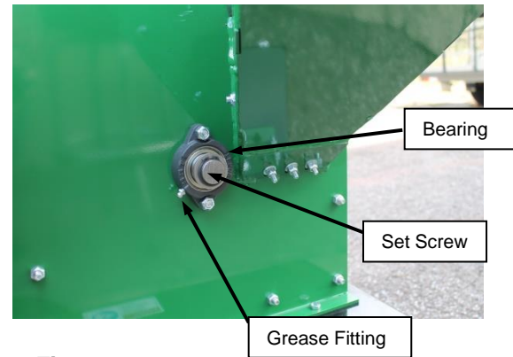
Figure 18 Front Chipper Bearing Shown
