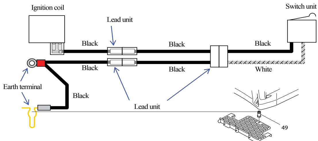
EB7650TH Wiring Diagram
