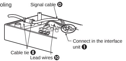
Card key coin timer connection
