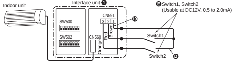
Card key coin timer connection
