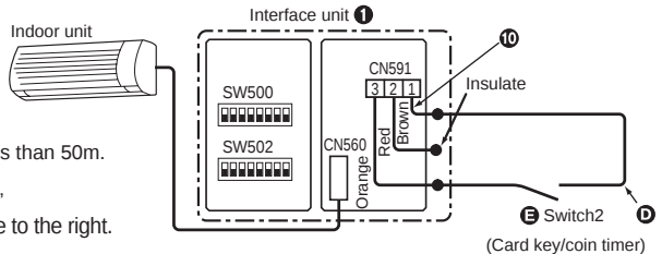
Card key coin timer connection
