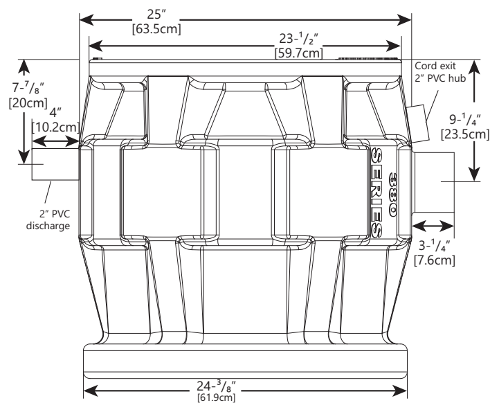
Figure 3. 380-Series Side Discharge Basin Dimensions
