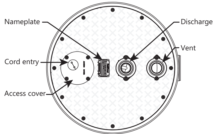
Figure 8. 700-Series Cover
