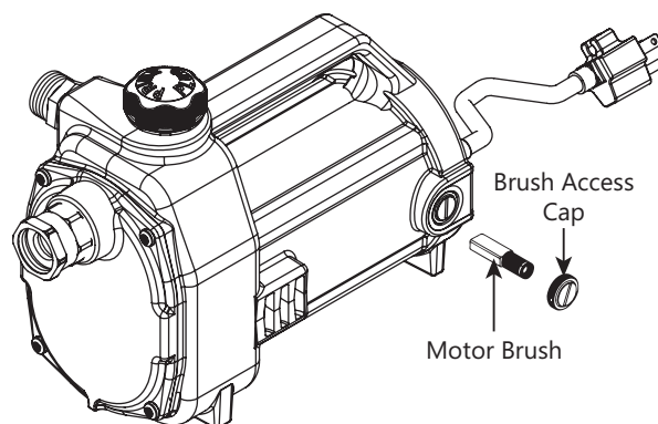
Figure 3. Motor Brush (only one side shown)
