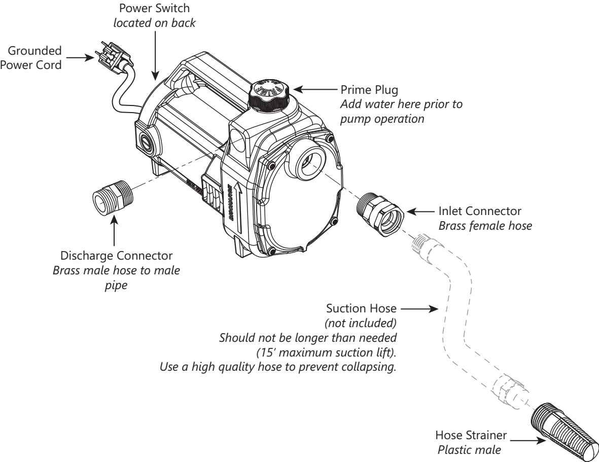
Figure 2. Transfer Pump Components
