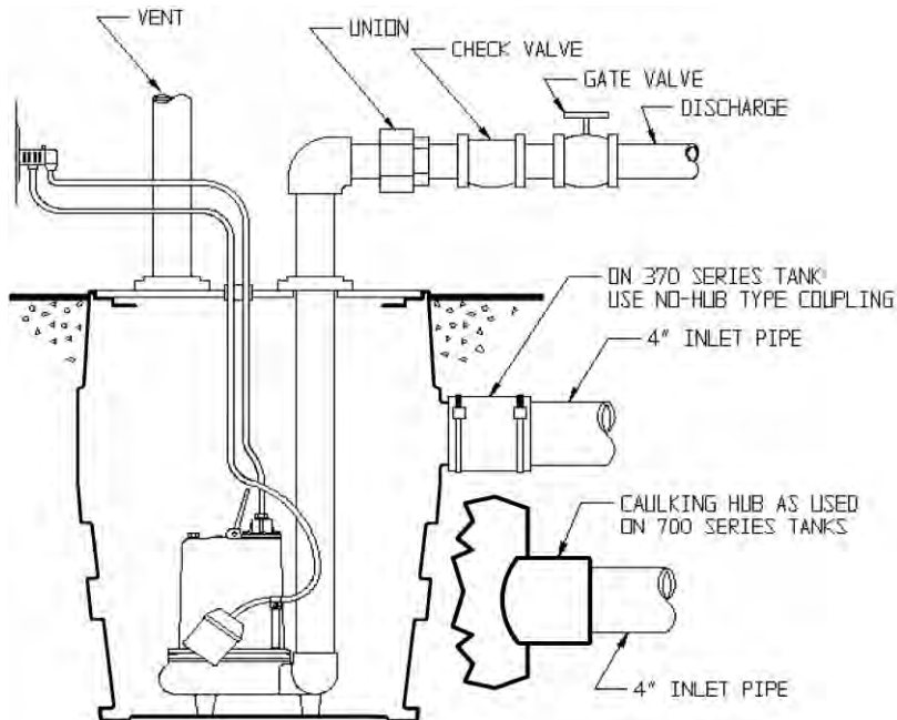
Fig. 2 – Typical Installation Simplex System This is a recommended installation only. Variations may apply.
