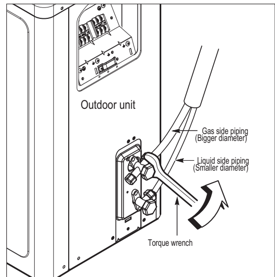
Figure 26: LAU180HYV1/LSU240HYV1 Outdoor Unit Piping Connection.
