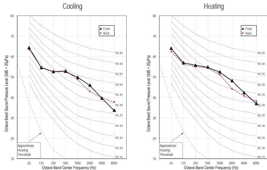
Figure 4: Sound Pressure Levels for LAU180-240HYV1 Outdoor Units.
