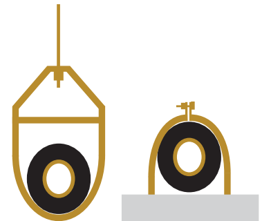
Figure 17: Pipe Hanger Details.
