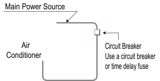
Figure 32: LAU180HYV1/LAU240HYV1 Outdoor Unit Electrical Connection.
