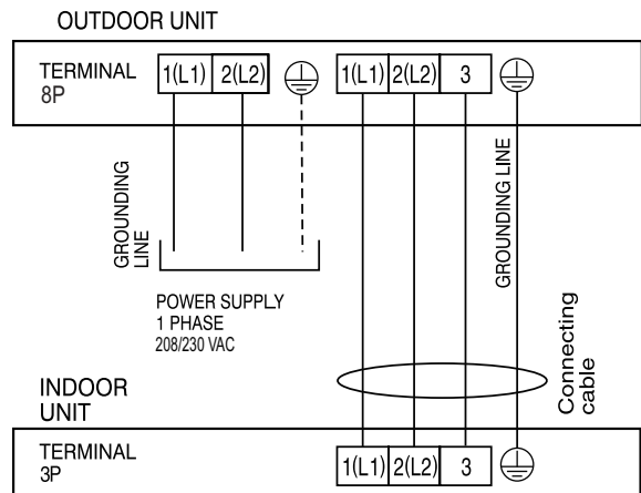
Figure 32: LAU180HYV1/LAU240HYV1 Outdoor Unit Electrical Connection.
