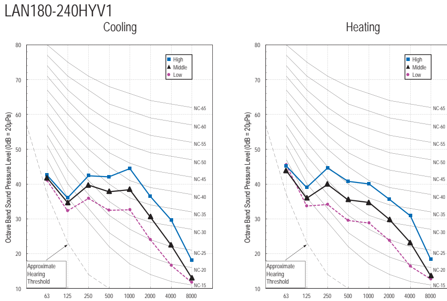
Figure 7: Sound Pressure Levels for LAN180-240HYV1 Indoor Units.
