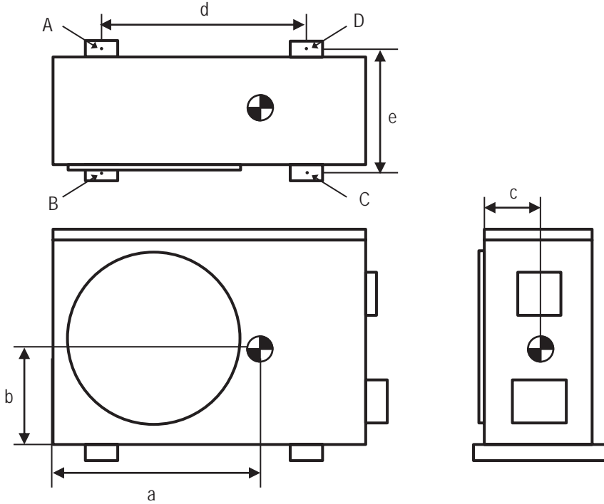
Figure 1: LAU090-240HYV1 Center of Gravity and Corner Weight Dimensions Diagram.
