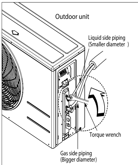
Figure 25: LAU090HYV1/LSU120HYV1 Outdoor Unit Piping Connection.
