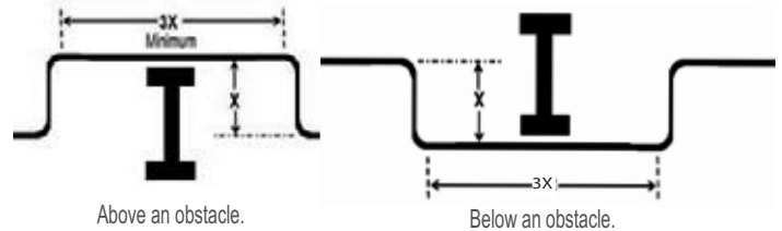
Figure 16: Installing Piping Above and Below an Obstacle.
