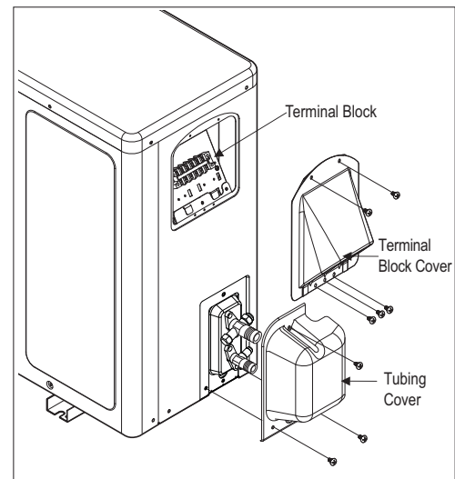
Figure 26: LAU180HYV1/LSU240HYV1 Outdoor Unit Piping Connection.
