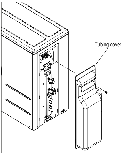
Figure 25: LAU090HYV1/LSU120HYV1 Outdoor Unit Piping Connection.
