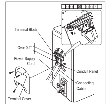
Figure 29: LAU180HYV1/ LAU240HYV1 Outdoor Unit Electrical Connection.
