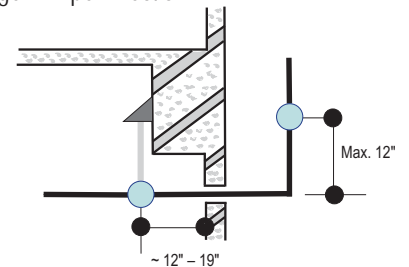
Figure 18: Typical Pipe Support Location—Change in Pipe Direction.
