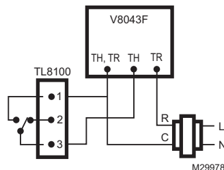
Fig. 8. Wiring diagram for a 24 VAC V8043F.
