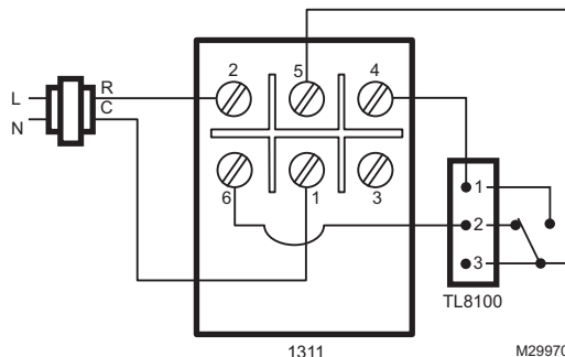
Fig. 9. Wiring diagram for a White Rogers 1311 valve.
