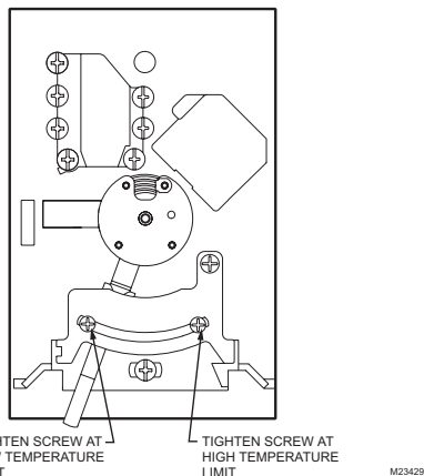
Fig. 3. Aligning range stop with thermostat.
