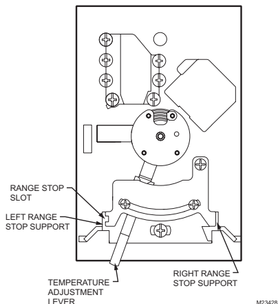
Fig. 2. Thermostat with front cover removed.
