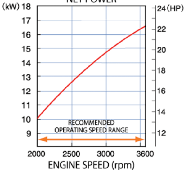
NET POWER
