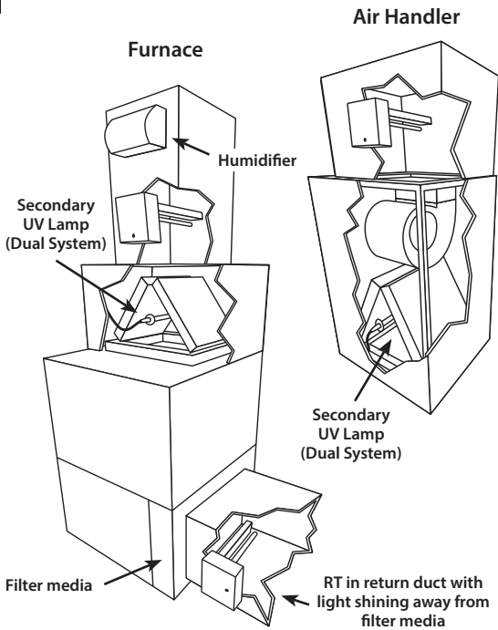
Main Unit
