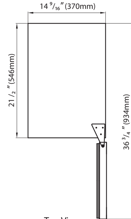
Top View
