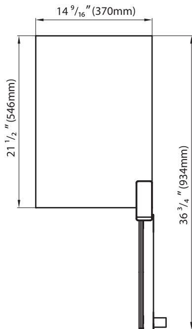
Cutout Height: 33 15/16"
