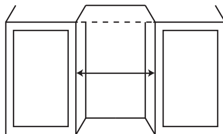
Cutout Width: 16 9/16"
