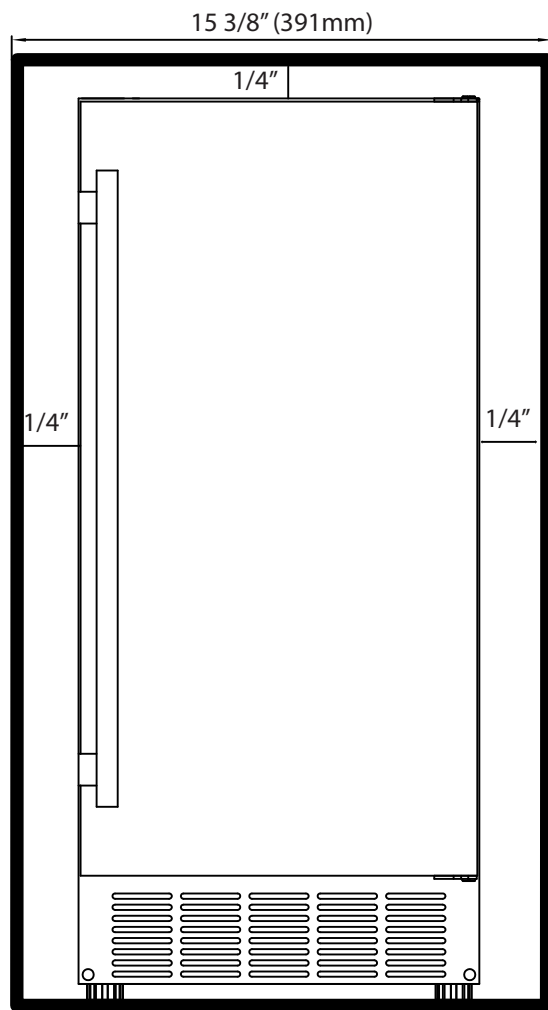
Front View
