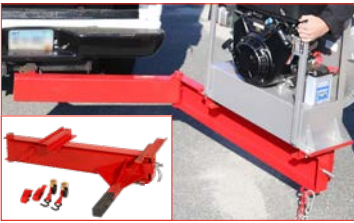
Hitch Mount Swing Arm
