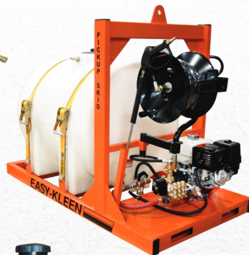
AS440GHGP/ES-SKID-225 with Pickup Skid and 225 Gallon Water Tank
