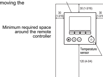
External dimensions of remote controller
