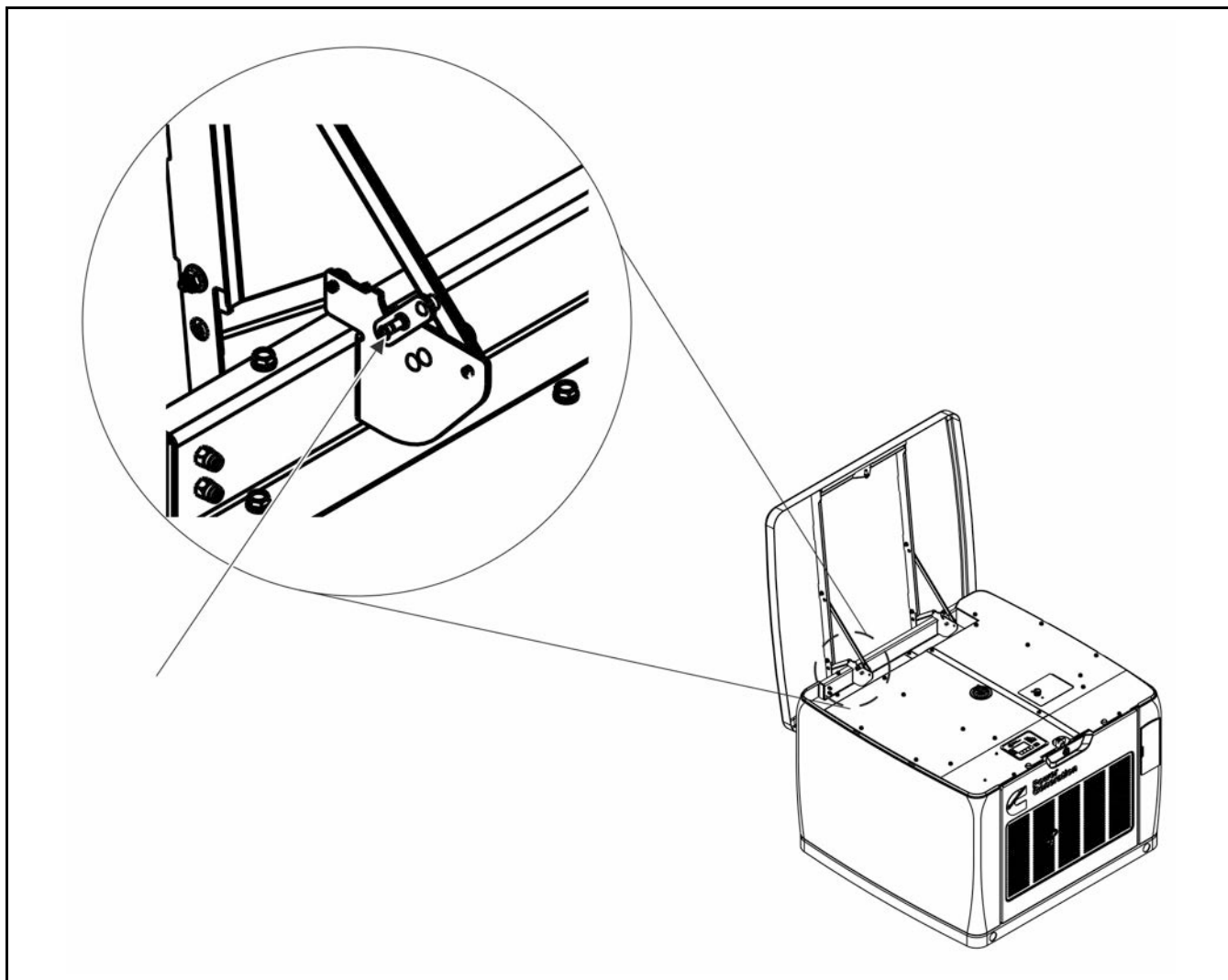
FIGURE 1. HINGE LOCATION
