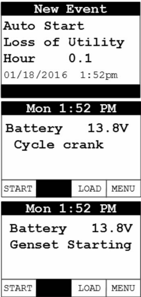
FIGURE 16. GENSET STARTING
