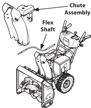
Overhead Chute Control (w/ Flex Shaft Steel Chute) Page 11
