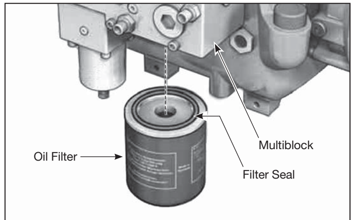
Figure 12 - Oil Filter
