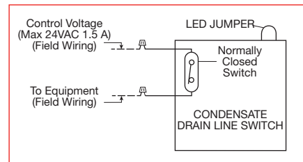
FIG. C: WIRING DIAGRAM
