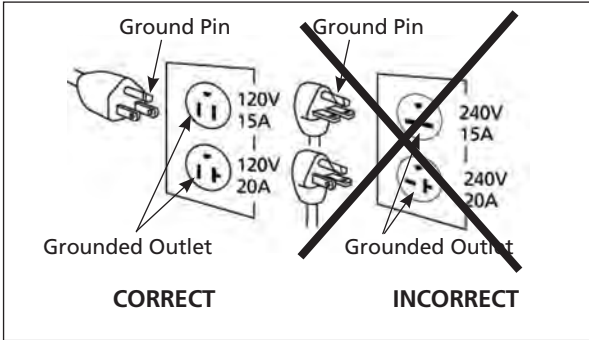
Figure 3 - Grounding Method
