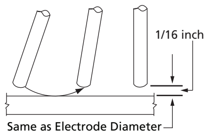
Figure 5 - Scratching Method
