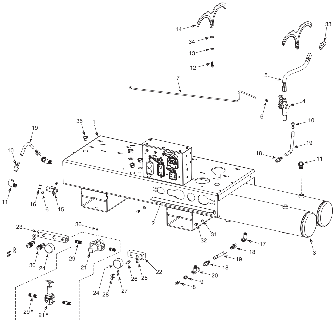
Figure 13 - Chassis Assembly for GR2100 and GR3100 shown; common parts for all models are detailed in Figure 13 parts list
