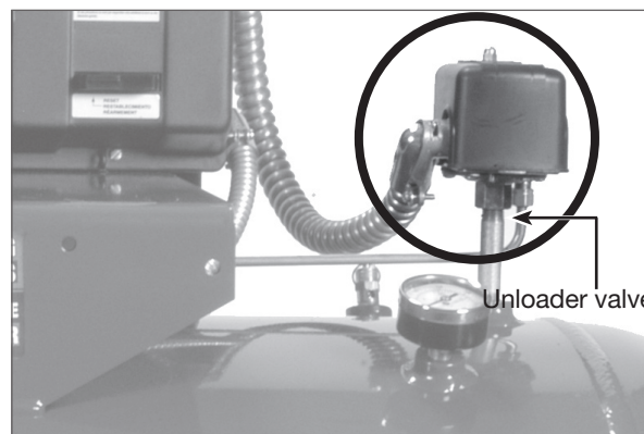
Figure 15 - Pressure Switch
