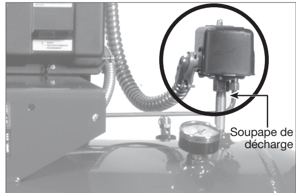
Figure 15 - Pressostat
