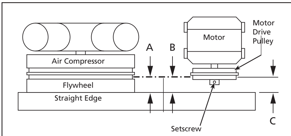
Figure 15 - Top View
