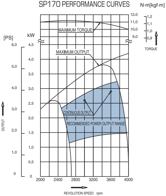
SP170 PERFORMANCE CURVES
