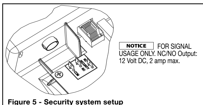
Figure 5 - Security system setup
