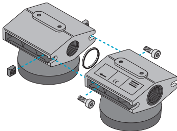
Filter connection kit allows easy mounting of filters in series (sizes 9-520)
