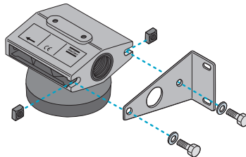
Wall mounting kit simplifies installation (sizes 9-520)
