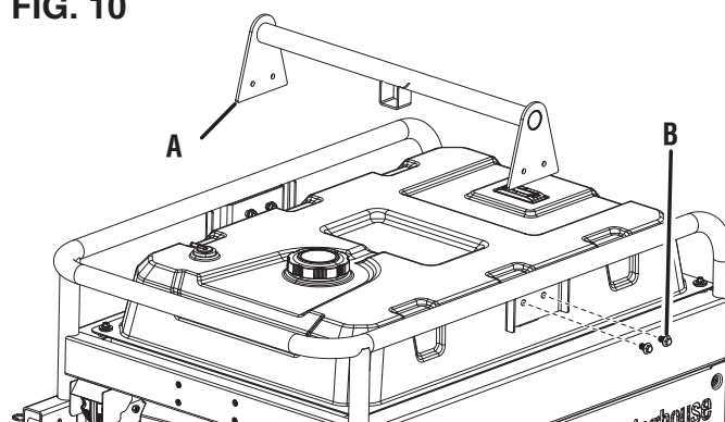
A - Support de levage B - Boulons
