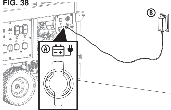
A - Battery charging port B - Charger
