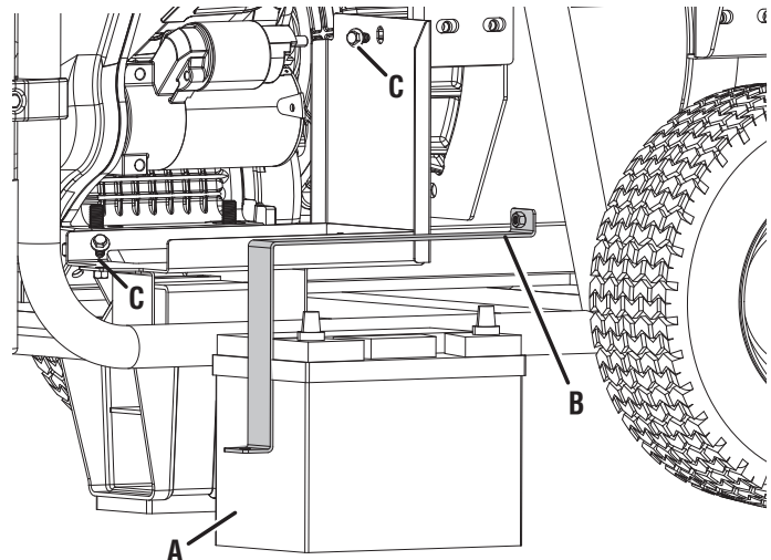
A - Battery B - Battery plate C - Bolt
