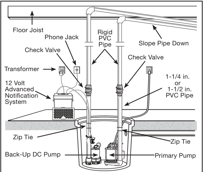
Figure 1 - Method 1 (Preferred Installation)
