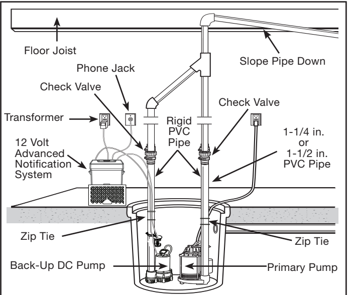
Figure 2 - Method 2 (Alternate Installation)
