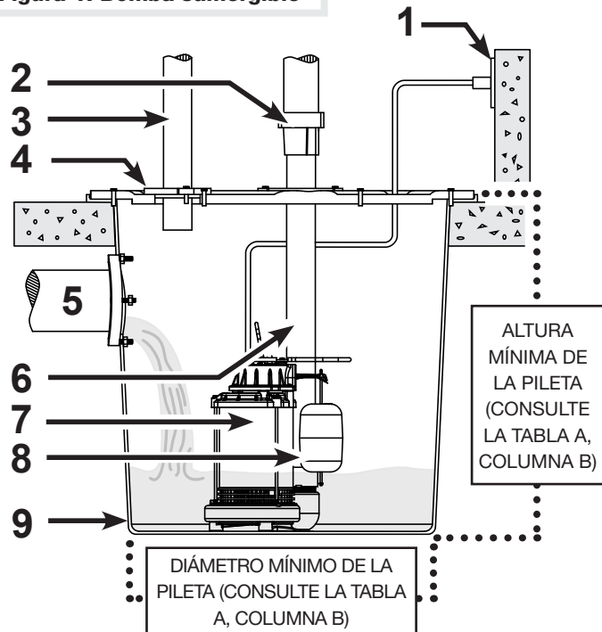
Figura 1: Bomba sumergible
