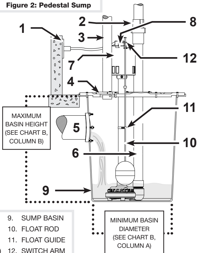
Figure 2: Pedestal Sump
