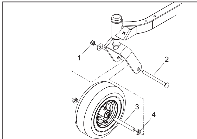
Caster wheels
