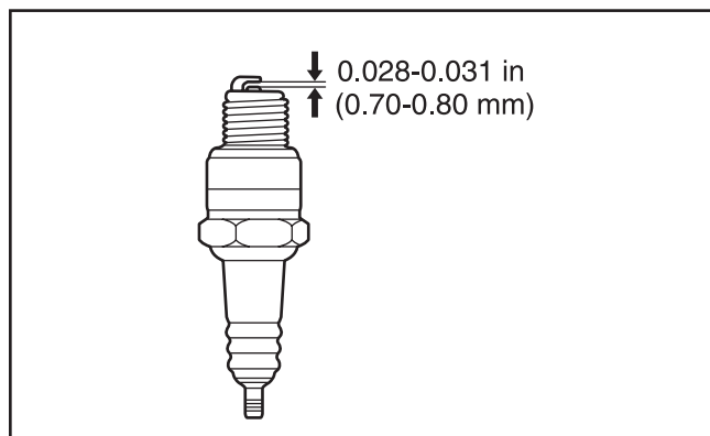
Measure the electrode gap
