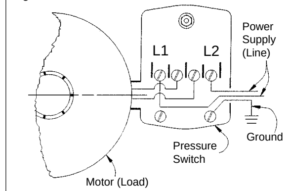
Fig. 1 Electrical Connections
