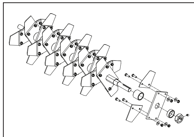
Delta blade
