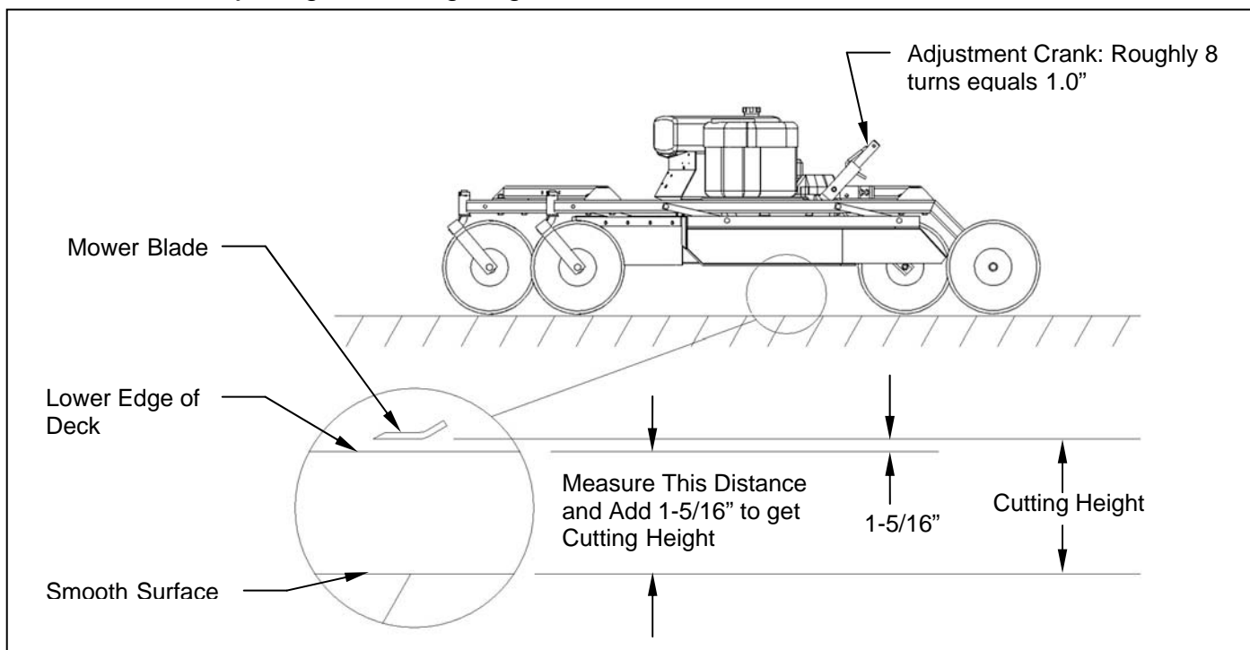
Figure 8: Adjusting Rough Cut Mower Cutting Height
