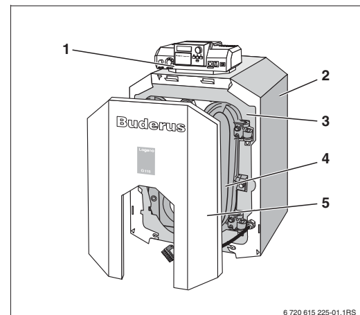
Fig. 1 Boiler without burner
