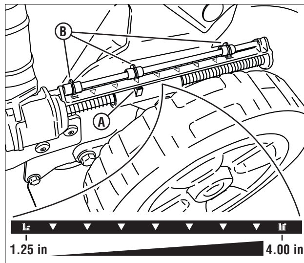
Figure 7: Cutting height indicator
