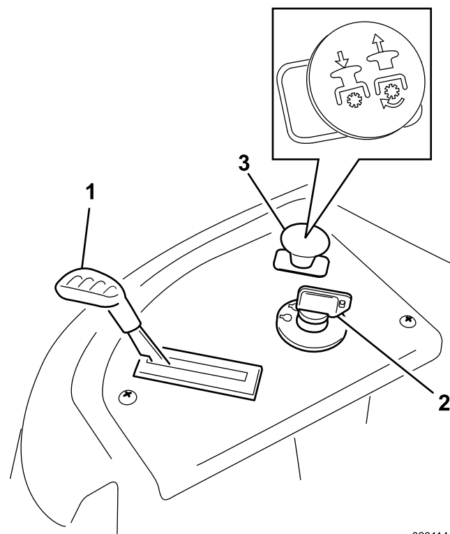
Figure 4 Control Panel
