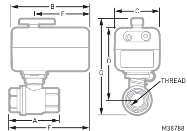
Fig. 1. Dimension diagram.
